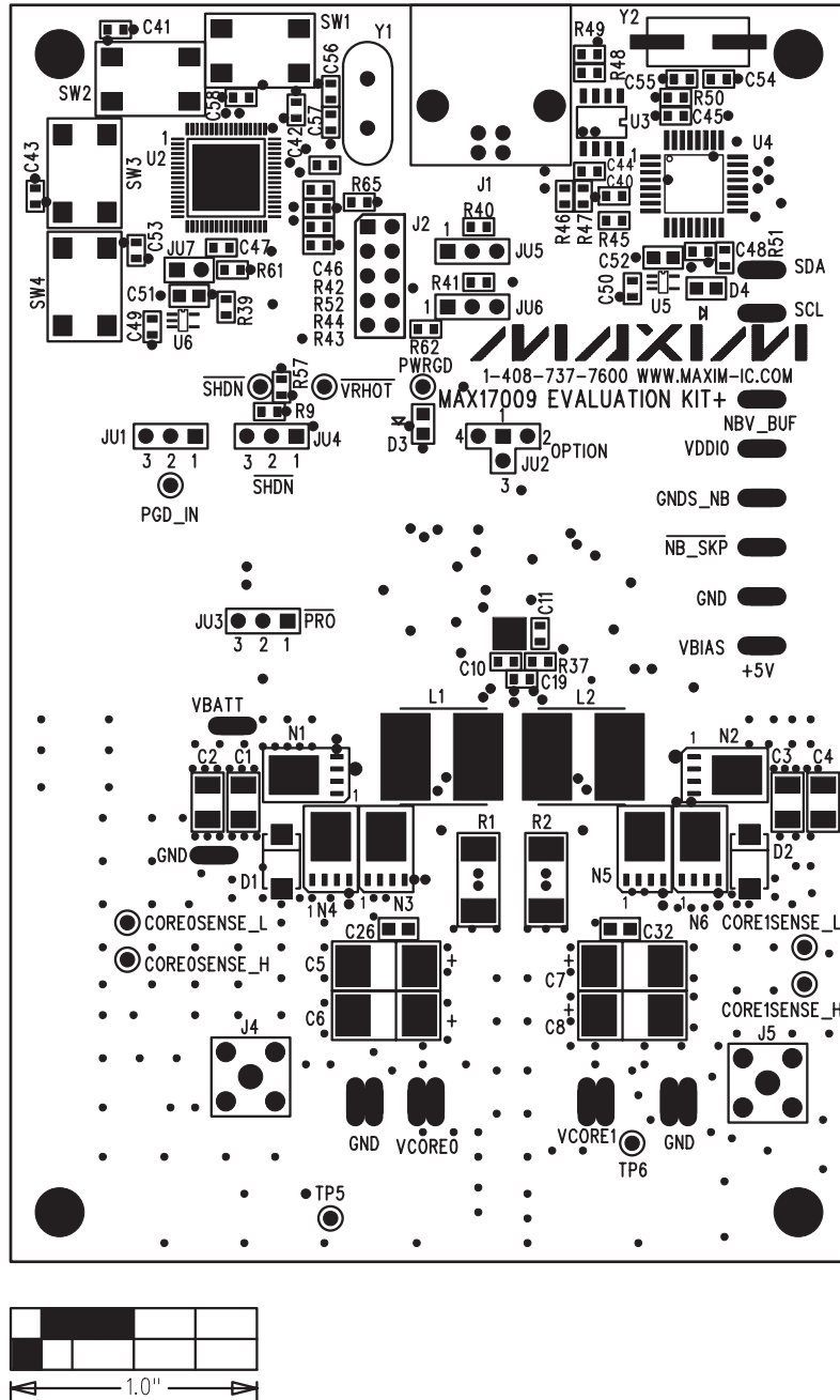
Figure 3. MAX17009 EV Kit Component Placement Guide—Component Side
