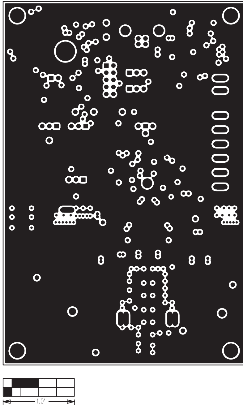
Figure 5. MAX17009 EV Kit PCB Layout—Internal Layer 2
