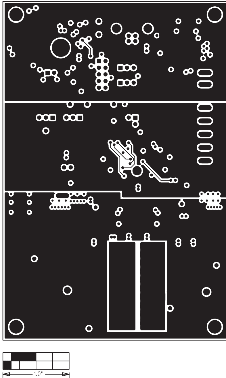
Figure 7. MAX17009 EV Kit PCB Layout—Internal Layer 4
