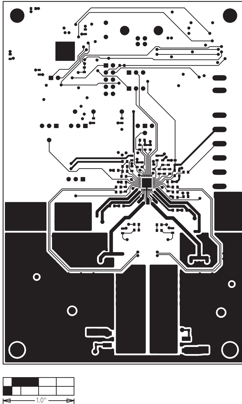
Figure 9. MAX17009 EV Kit PCB Layout—Solder Side
