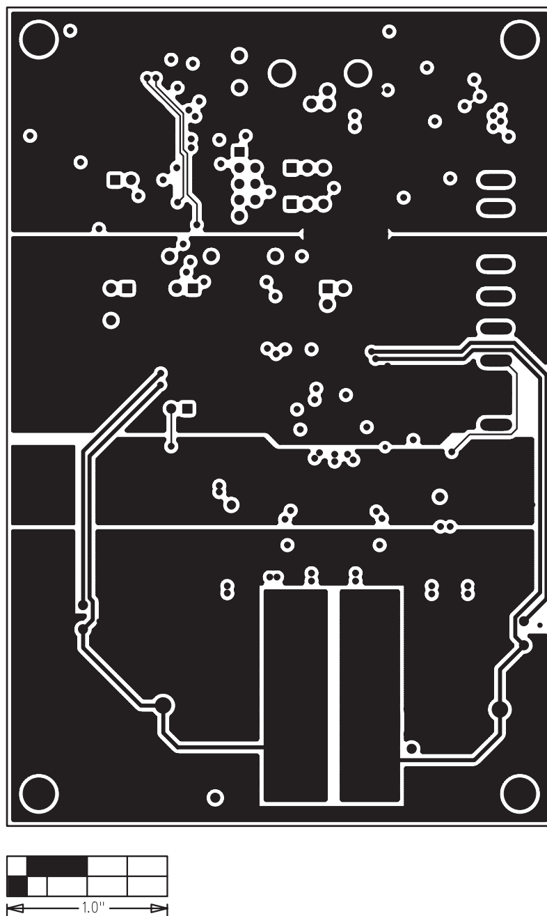
Figure 6. MAX17009 EV Kit PCB Layout—Internal Layer 3
