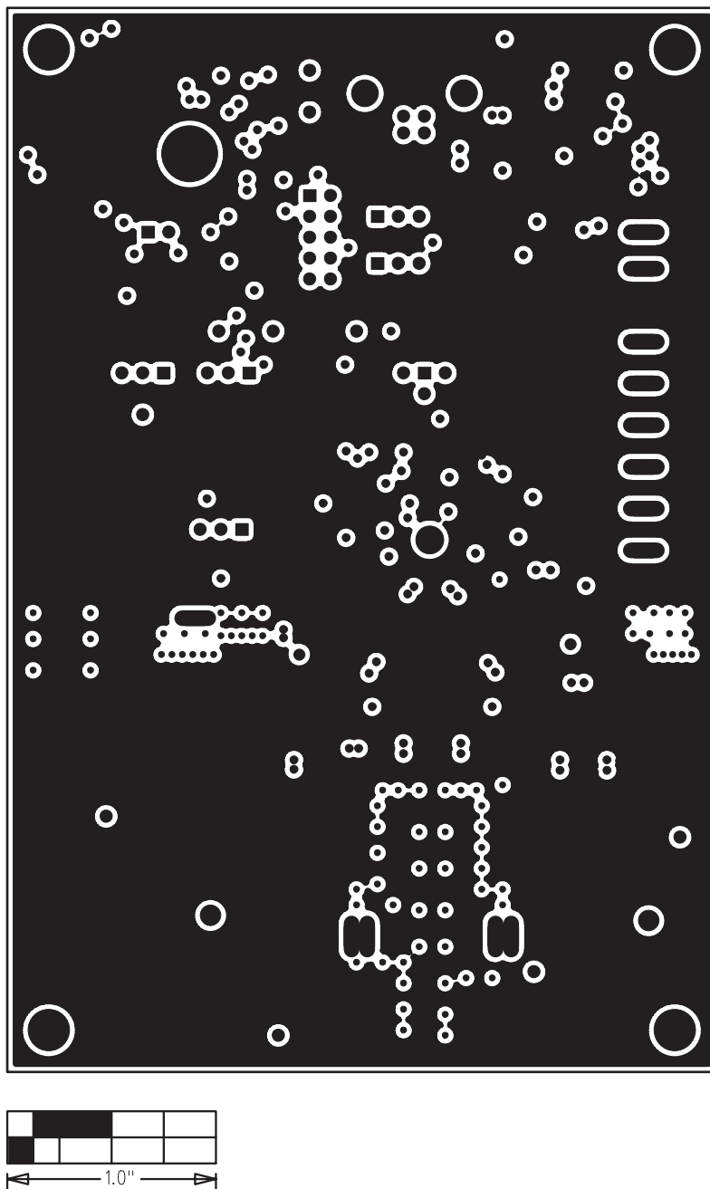
Figure 8. MAX17009 EV Kit PCB Layout —Internal Layer 5
